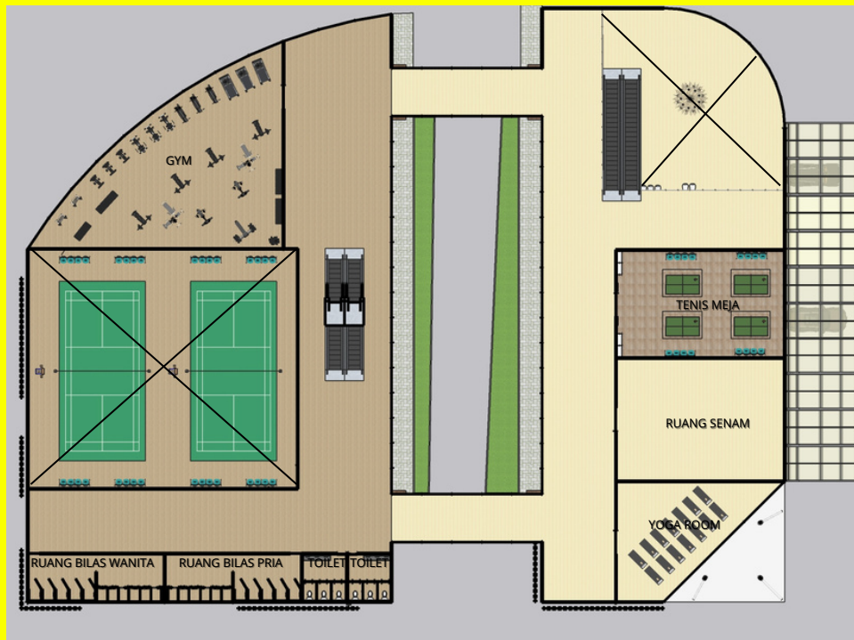
DENAH LANTAI 2
